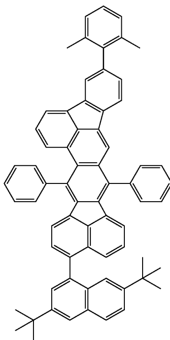
Synthesis example 21
