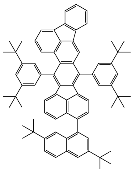
Synthesis example 9
