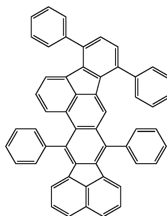
Synthesis example 26
