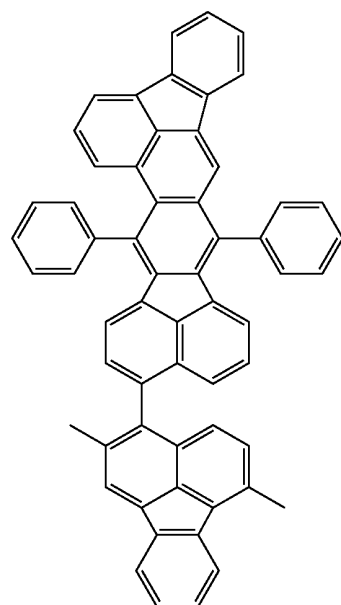
Synthesis example 24
