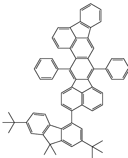
Synthesis example 28
