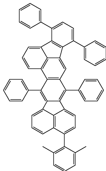
Synthesis example 27
