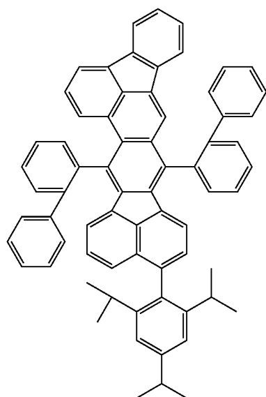
Synthesis example 11
