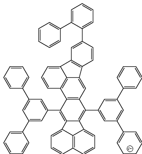
Synthesis example 22
